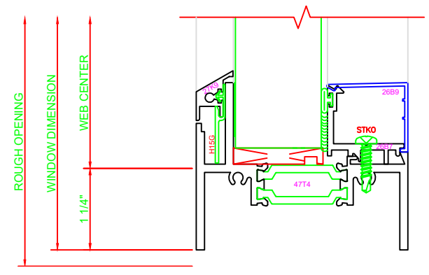
200 SILL SERIES: 321G FIXED
