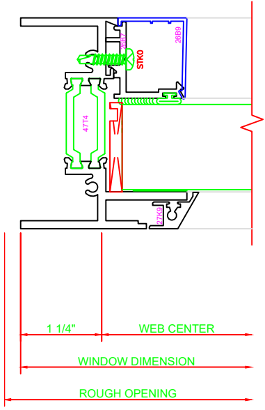
400 JAMB SERIES: 321G FIXED
